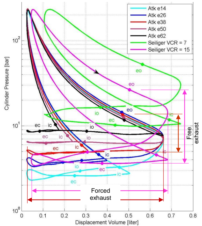
Figure 3A Cylinder pressure (logarithmic) - displacement volume ( p, V ) diagrams with valves timing for all cycles
