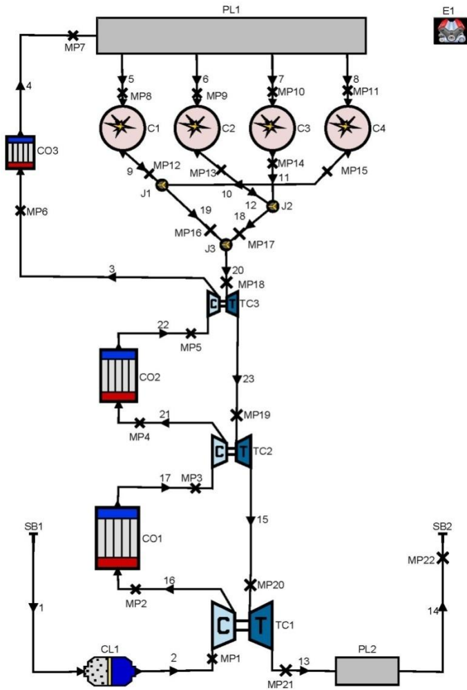
Figure 1 BOOST model of a four cylinder TC engine Simple number denotes pipes, Cx = cylinder, COx = cooler, TCx = turbochargers, PLx = plenum, Jx = junctions, CLx = cleaner, SBx = system boundaries, Ex = engine and MPx = measuring points
