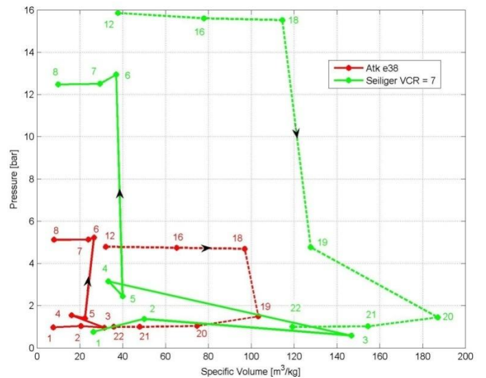
Figure 4A Pressure - specific volume ( p, v ) diagrams for some MP from the intake (solid lines) and exhaust (dashed lines) pipes for two selected cycles
