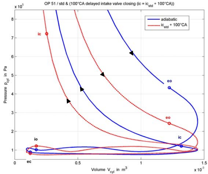
Figure 4 Pressure-Volume diagram (SV & IV)
