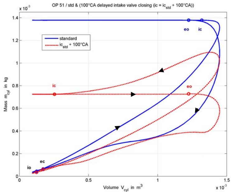
Figure 5 (gas mixture) Mass-Volume diagram (SV & IV)
