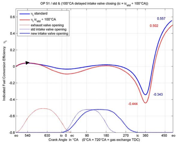
Figure 7 (indicated fuel conversion) Efficiency–Crank Angle diagram (SV & 2V)
