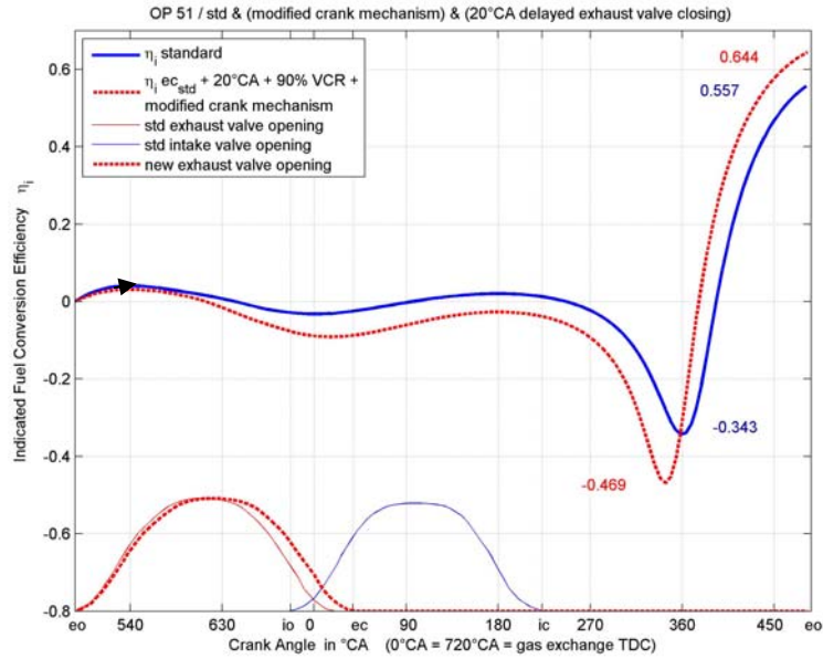
Figure 14 (indicated fuel conversion) Efficiency–Crank Angle diagram (SV & 3V)
