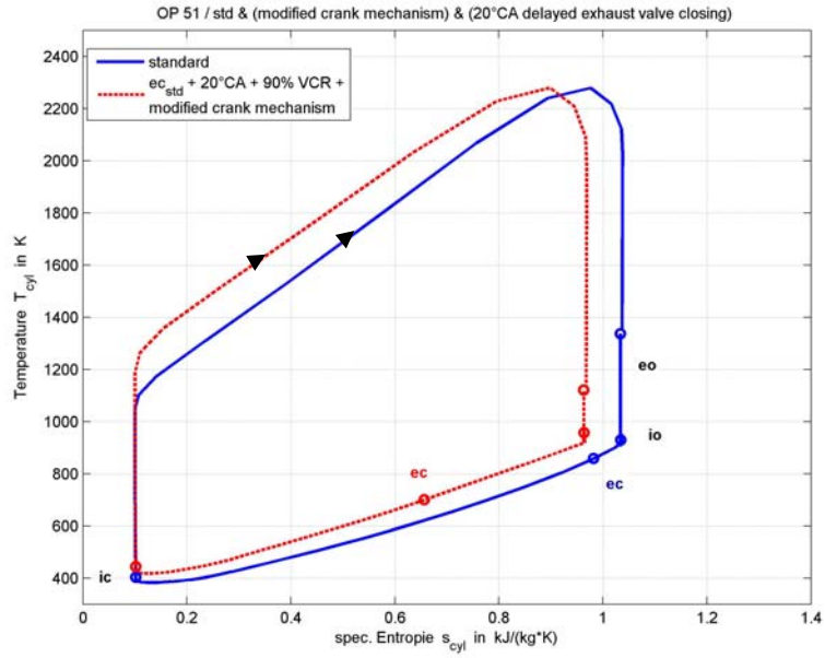
Figure 12 Temperature-(specific) Entropy diagram (SV & 3V)
