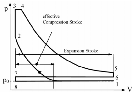
Figure 2. Schematic Pressure-Volume diagram of a modified (i.e. four stroke) Atkinson cycle
