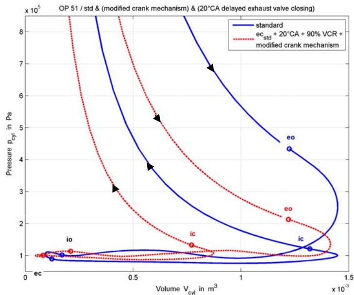
Figure 11 Pressure–Volume diagram ( SV & 3V )
