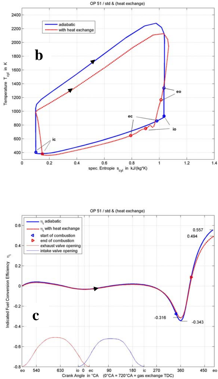
Figure 3 Comparison between adiabatic (SV) and non-adiabatic cycles
