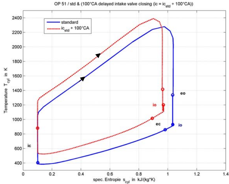
Figure 6 Temperature-(specific) Entropy diagram (SV & IV)
