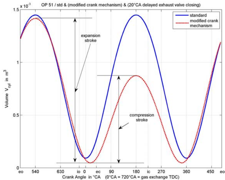
Figure 10 Volume-Crank Angle diagram (SV & 3V)
