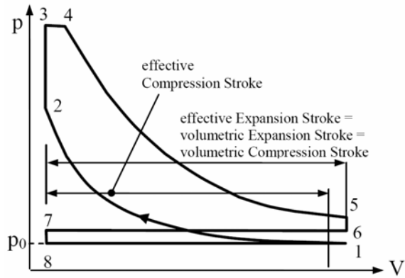
Figure 1. Schematic Pressure-Volume diagram of a classical four stroke cycle of conventional ICE
